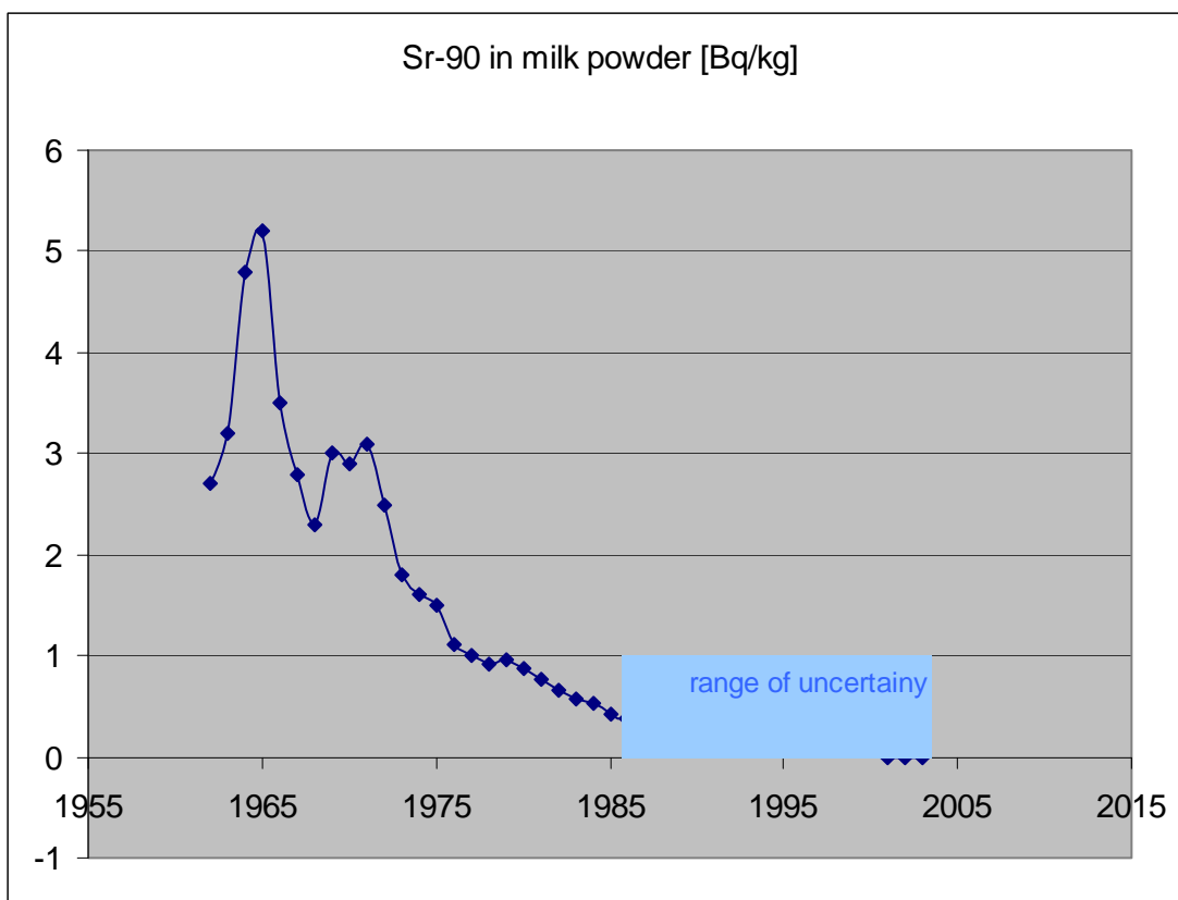
Figure 1: Sr-90 in New Zealand milk powders
